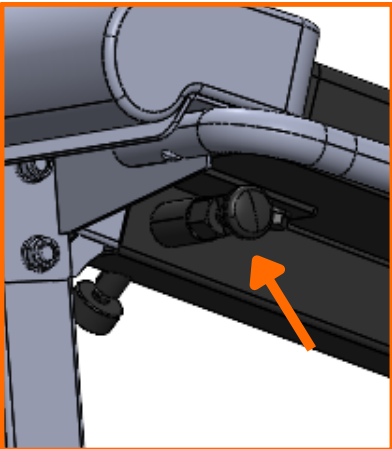
4. Use this Pin to lock the LD to the ABX
